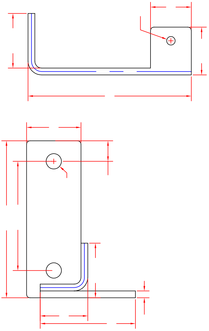
ELEVATION VIEW
