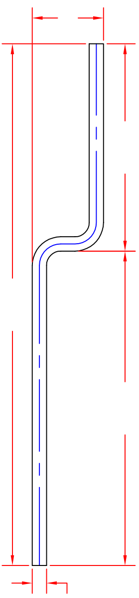
ELEVATION VIEW
